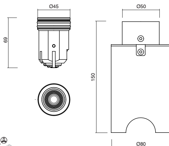
HOUSING/ CONTROCASSA
