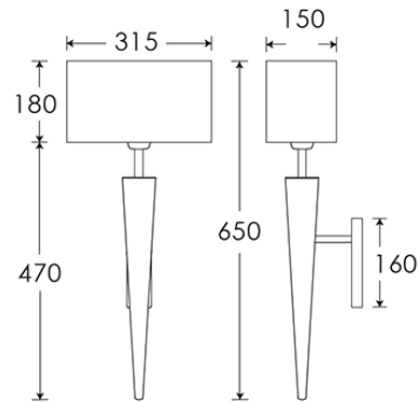
Dimensions in mm and approximate
