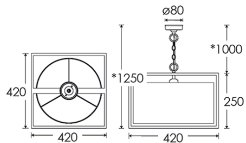
Dimensions in mm and approximate *Adjustable flex and chain length
