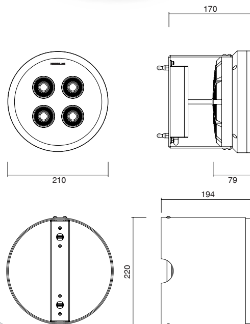
HOUSING/ CONTROCASSA
