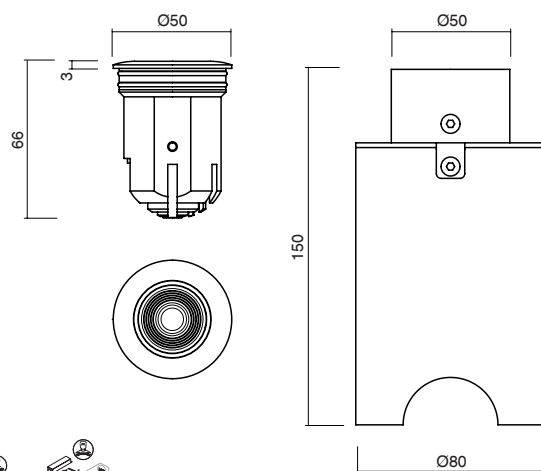
HOUSING/ CONTROCASSA
